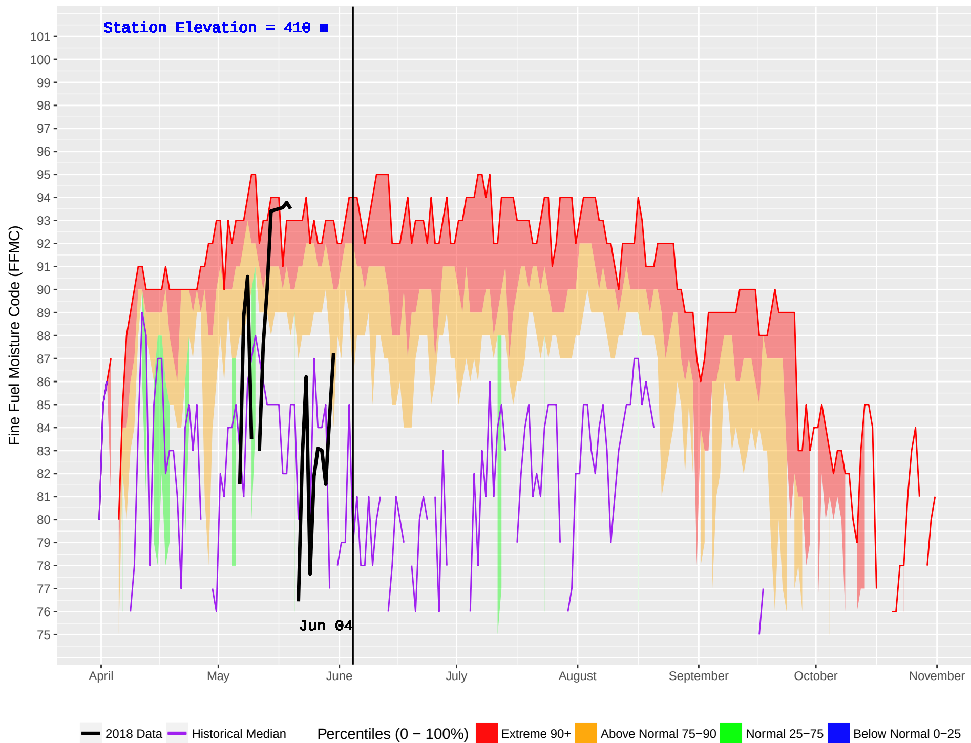
UPPER KISPIOX (431) : Historical (1986–2016) and Current (2018) Noon Fine Fuel Moisture Code (FFMC)
